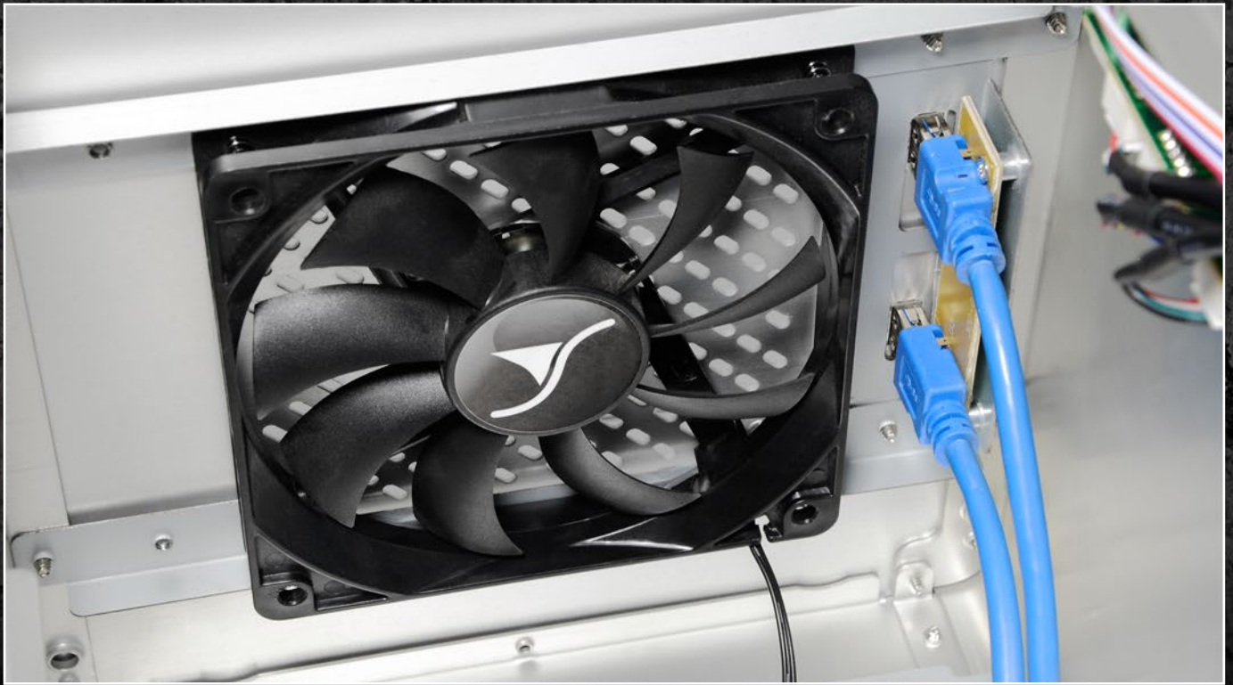
120 mm fan pre-installed to the top panel
